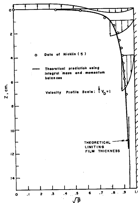
Fig. 4. Bubble shape ( \sqrt{\beta} vs. Z ) and velocity profiles in the liquid film for the numerical example of Nicklin.
