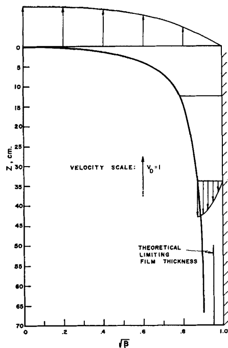
Fig. 9. Bubble shape ( \sqrt{\beta} vs. Z ) and velocity profiles in the liquid film in a continuously flowing air-water system.
