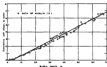
Fig. 6. Cumulative wall shear acting on the liquid film vs. bubble length for the numerical example of Nicklin.
